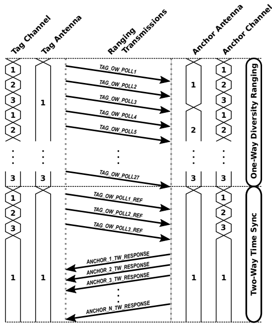
Figure 1: Ranging protocol. PolyPoint is able to leverage antenna diversity without significantly impacting position update rate. The protocol starts with a series of 27 broadcast transmissions from the tag for each combination of tag antenna, anchor antenna, and RF channel. The time-of-arrival data collected from this sequence provides information on the difference between all range estimates throughout the sequence. Finally, a two-way time-of-flight handshake is sent (on each channel for robustness) to determine the true range estimate—a total of 30 POLL messages. The offset between the first and last poll message on each channel is used to calculate the crystal frequency offset between the tag and anchor. From the first measurement, the time offset between the tag and anchor is known, leading to estimates of range for the other 26 combinations from the initial difference-based measurements.
